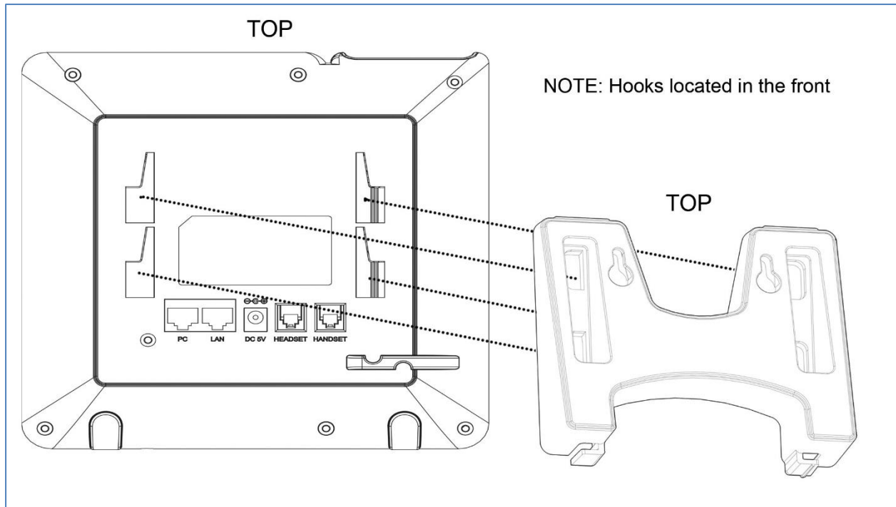
Figure 3: GXP16xx Wall Mount installation
